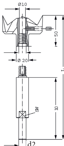
110-130mm / M16 / Schaft / Queue 16mm
